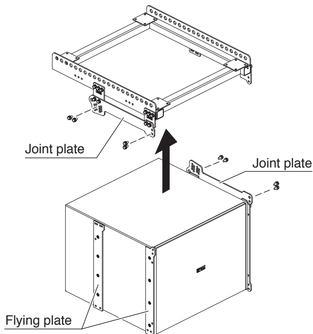
Subwoofer assembly diagram
