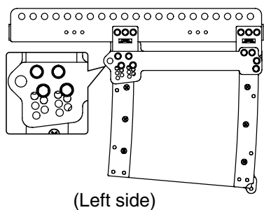
Subwoofer finished assembly diagram
