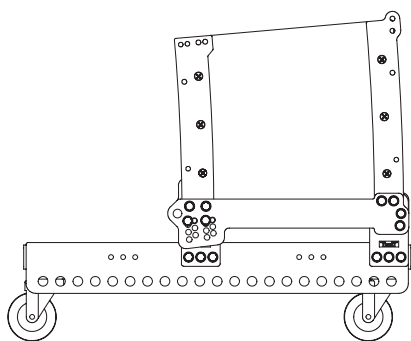
Subwoofer finished assembly diagram
