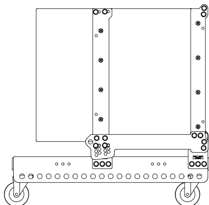
Subwoofer finished assembly diagram
