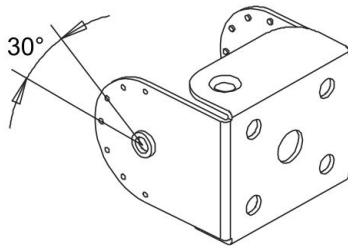
[Speaker bracket]
