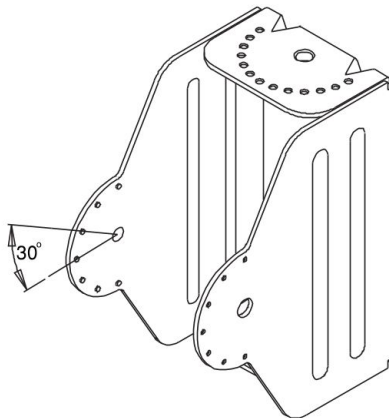
[Speaker bracket]
