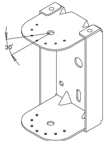
[Wall bracket]
