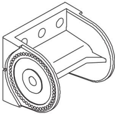
[Rear mount block]
